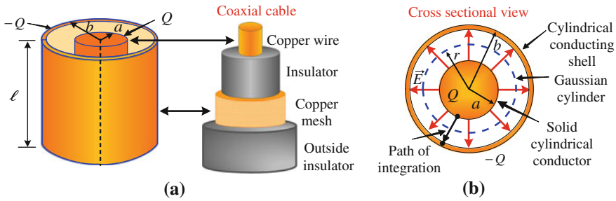
Fig. 23.3 (a) A cylindrical capacitor in the form of a cylindrical solid conductor surrounded by a coaxial shell. (b) A cross-sectional view of the capacitor showing a Gaussian cylinder of radius a < r < b
