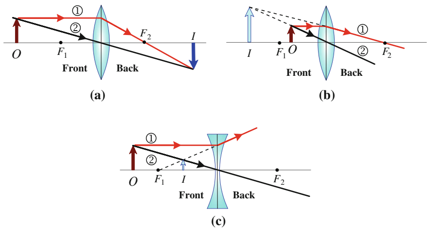
Fig. 17.24 Ray diagrams for locating the image formed by a thin lens. (a) An object in front of a converging lens (double convex lens). When the object is outside the focal point, the image is real, inverted, and on the back side of the lens. (b) When the object is between the focal point and the converging lens (double convex lens), the image is virtual, upright, larger than the object, and on the front side of the lens. (c) When an object is anywhere in front of a diverging lens (double concave lens), the image is virtual, upright, smaller than the object, and on the front side of the lens
