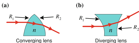
Fig. 17.21 (a) An enlargement of the top part of a converging lens. (b) An enlargement of the top part of a diverging lens
