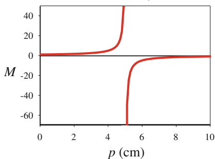
(a) Concave mirror ( f = 5 cm)
