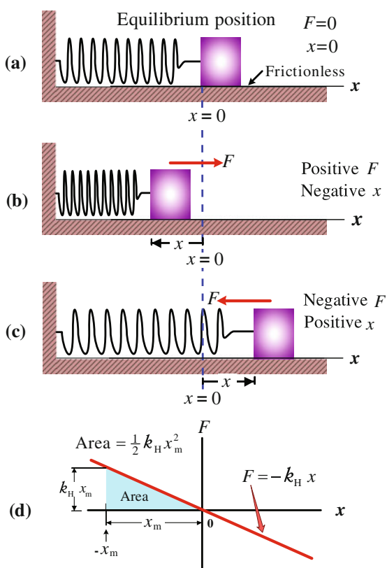
Fig. 6.8 The variation of the force of a spring on a block.
