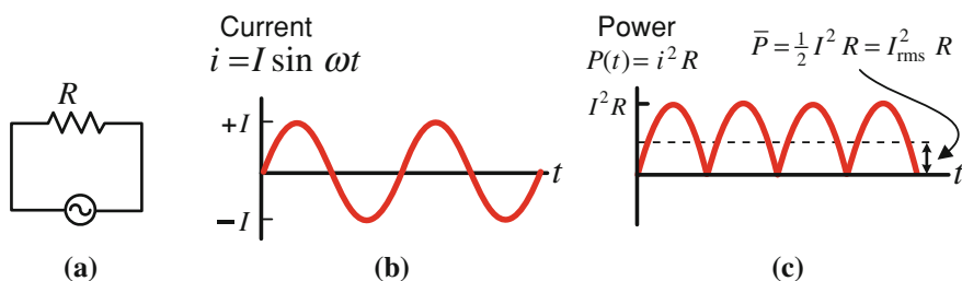
Fig. 27.10 (a) A resistor connected to an ac source. (b) Alternating current in a resistor as a function of time. (c) Power and average power delivered to a resistor as a function of time
