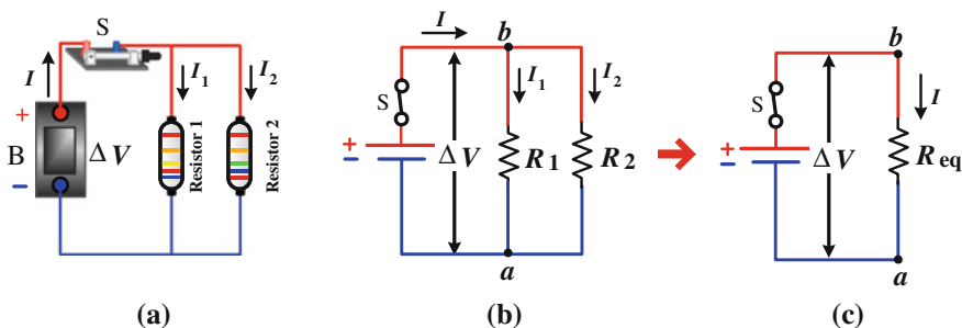
Fig. 24.15 (a) Two resistors of resistances R_1 and R_2 are connected in parallel to a battery B that has a potential difference \Delta V . (b) The circuit diagram for this parallel combination. (c) The equivalent resistance R_{\text{eq}} replacing the parallel combination
