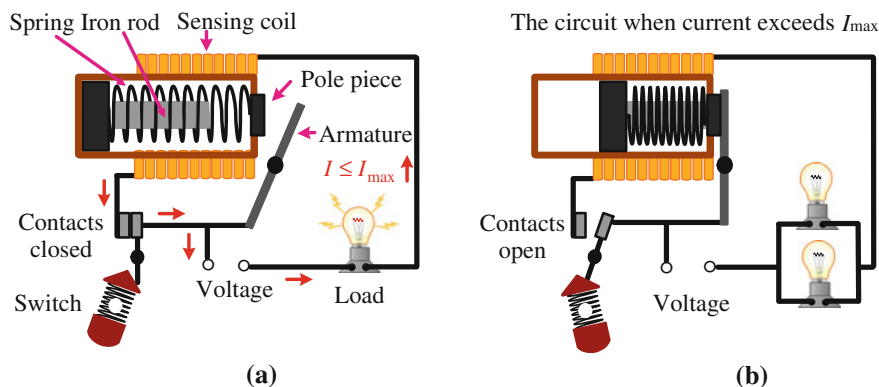
Fig. 26.20 (a) The circuit breaker is closed when the current I is maximum, I = I_{\max} , or even when I \leq I_{\max} . (b) When I exceeds I_{\max} , the armature unlatches a trip mechanism, and the circuit is opened
