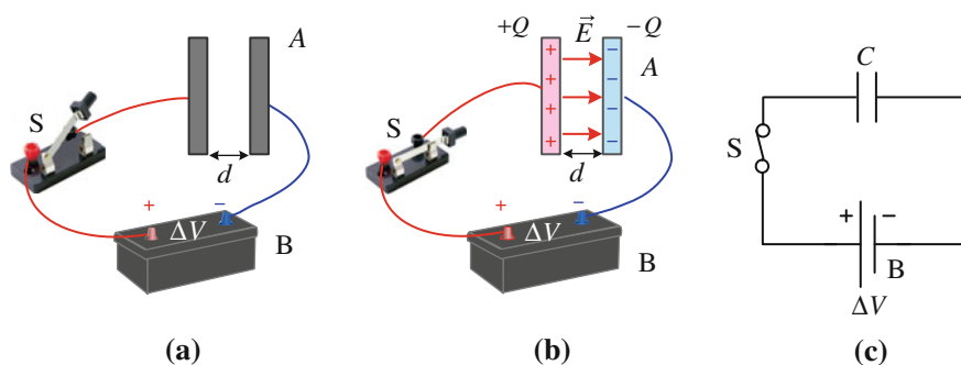
Fig. 23.2 (a) A parallel-plate capacitor is connected to a battery B and an open switch S . (b) When S is closed, each capacitor plate will carry equal but opposite charges of magnitude Q . (c) A schematic diagram of the circuit with symbols representing the elements used
