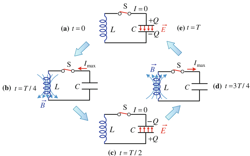
Fig. 28.11 (a) At t=0 , all of the energy is stored as an electric energy Q^2/2C in the capacitor. (b) At t=T/4 , all of the energy is stored as a magnetic energy \frac{1}{2}LI_{\max}^2 in the inductor. (c) At t=T/2 , all of the energy is stored again in the capacitor, but with opposite polarity. (d) At t=3T/4 , all of the energy is stored as a magnetic energy \frac{1}{2}LI_{\max}^2 in the inductor. (e) At t=T , the circuit returns to its initial configuration at t=0
