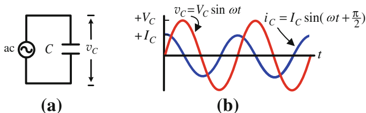
Fig. 28.18 (a) A capacitor connected to an ac source. (b) Alternating voltage v_C (red) lags alternating current i_C (blue) by quarter a cycle or 90^\circ
